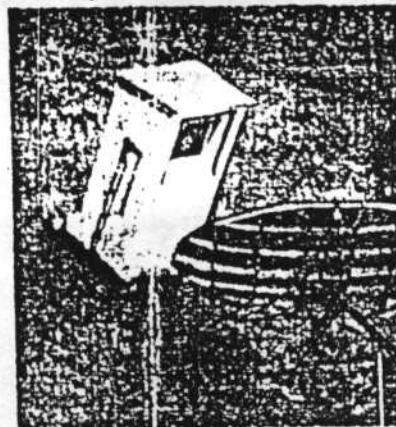
Reflector for heating water stored in an insulated tank.
