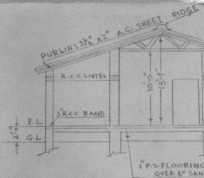
SECTION ON A
