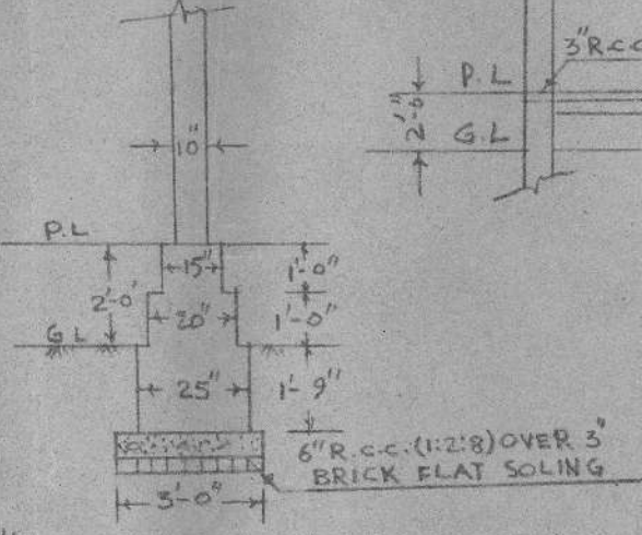
DETAIL OF FOUNDATION
