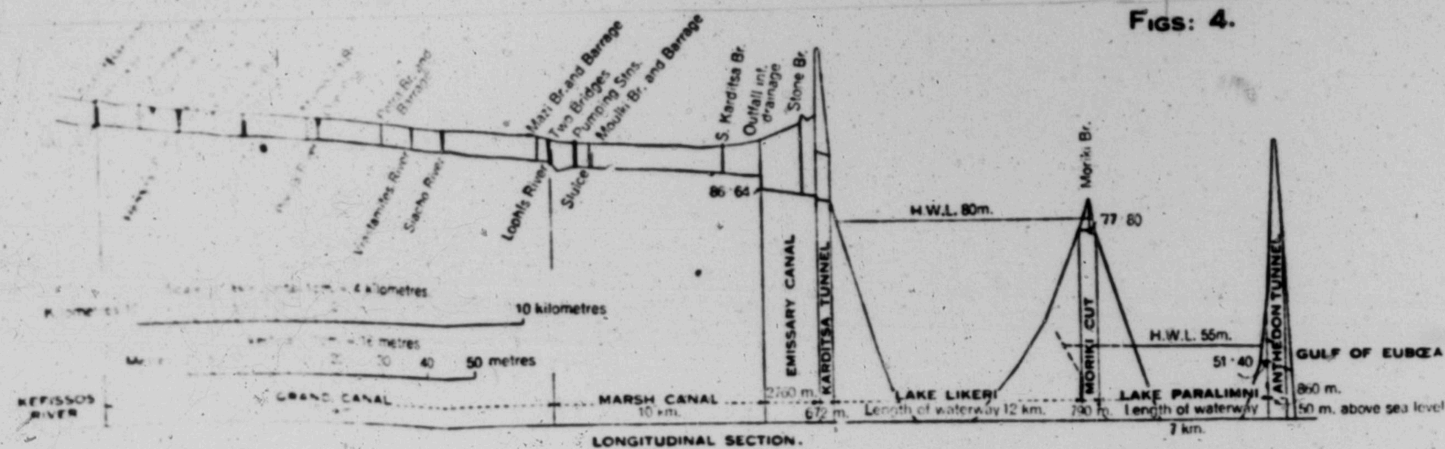
EXTERIOR DRAINAGE-WORKS FROM KEFISSOS RIVER TO THE SEA.
