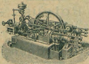
Zwillings-Dampf-Presspumpe.
